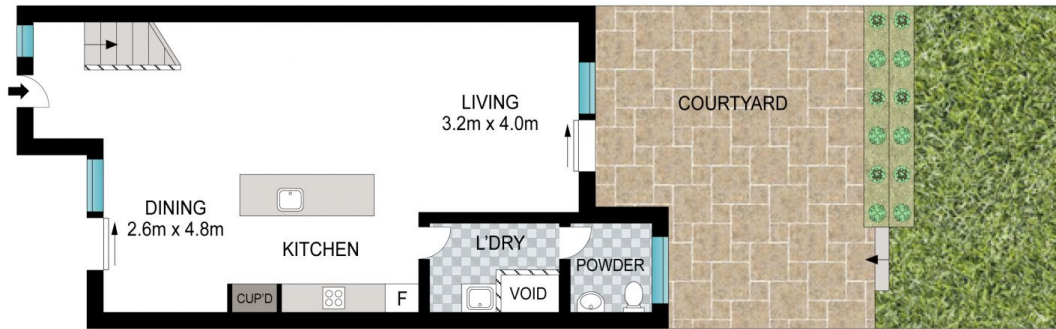
GROUND FLOOR
